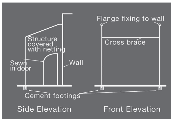
Figure 7: Tubular steel enclosure
