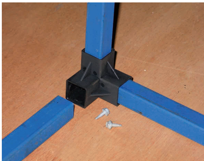
Figure 1: Prefab frame fitting
