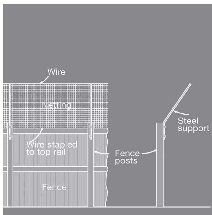
Figure 3: Completed steel support with netting
