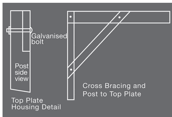
Figure 3: Top plate housing
