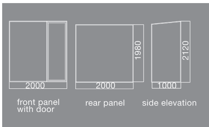
Figure 2: Steel frame for base unit
