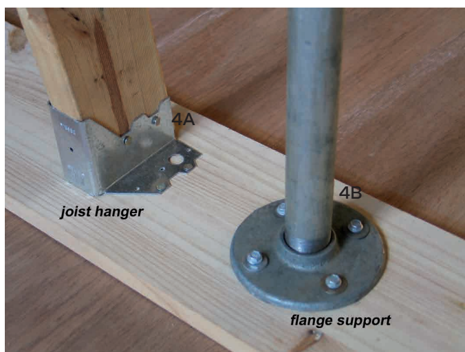
Figure 4A: Fixing method for timber Figure 4B: Fixing method for galvanised steel tubing
