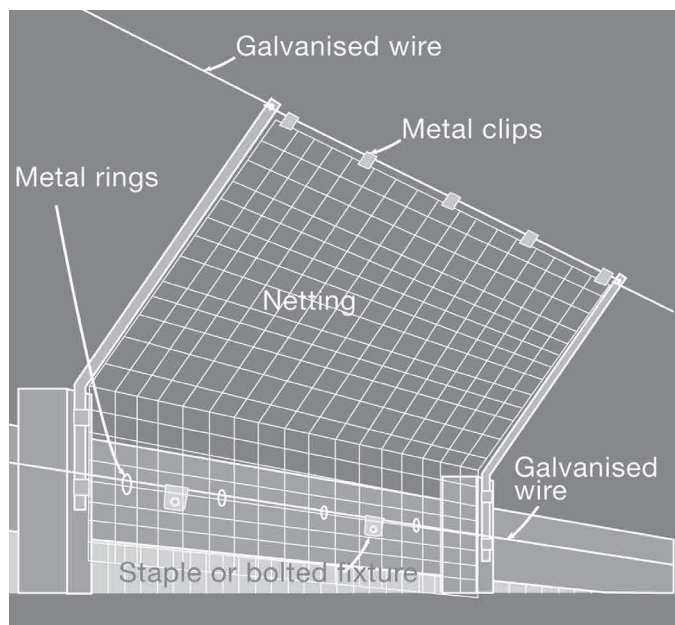
Figure 5: Securing the netting
