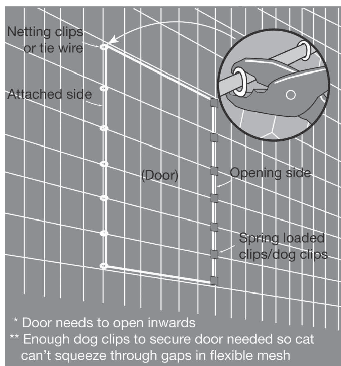
Figure 8: Design and construction of door
