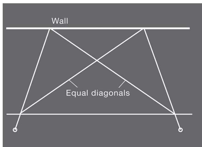
Figure 2: String line set out
